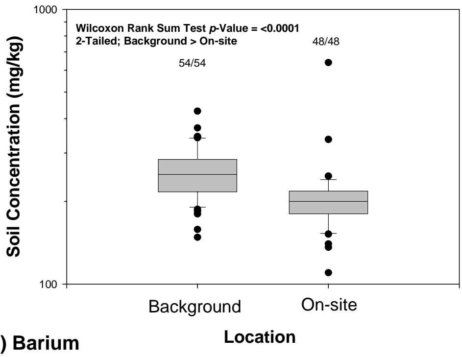
Figure B-3. Comparison of distributions of on-site and background concentrations of a) arsenic and b) barium at the Thermal Treatment Unit, Hill Air Force Base, Utah. On-site data includes samples through 2004.
